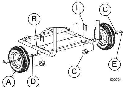
Figure 2-8. Wheel Assembly
