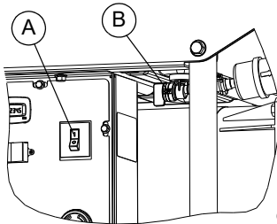
Figure 3-2. Main Breaker Switch and Fuel On/Off Valve
